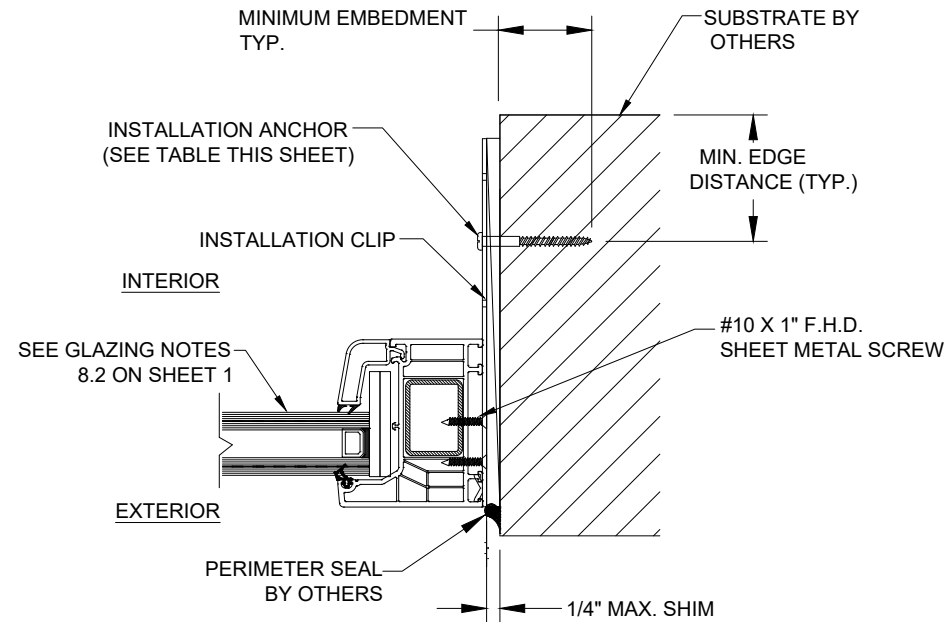
C 4 ANCHOR DETAIL INSTALLATION CLIP FRAME JAMB
